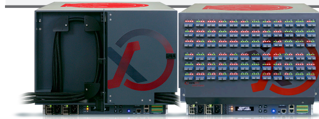
► XSOS-576D units: 576DS (left) – duplex, spliced connection; 576D (right) – duplex connection
